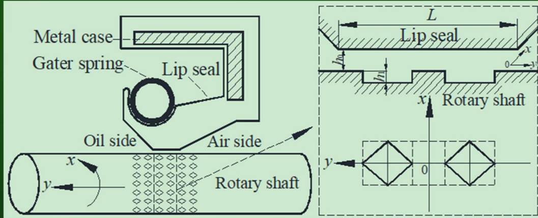
Fig.1 Schematic of the lip seal structure and local profile
