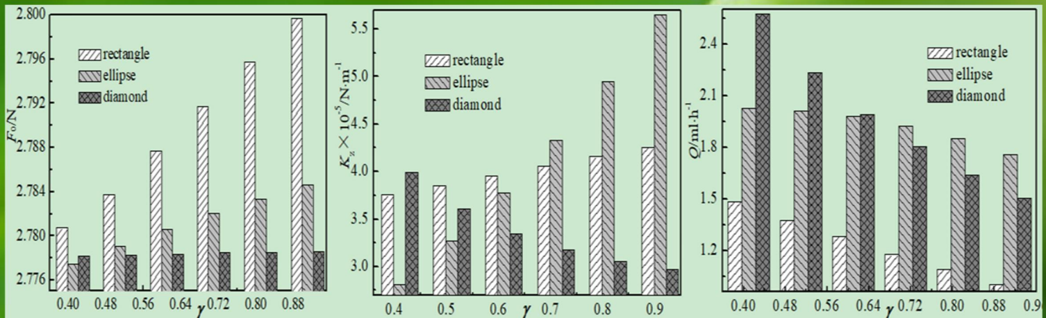
Fig.3 Effect of \gamma on sealing performance parameters
