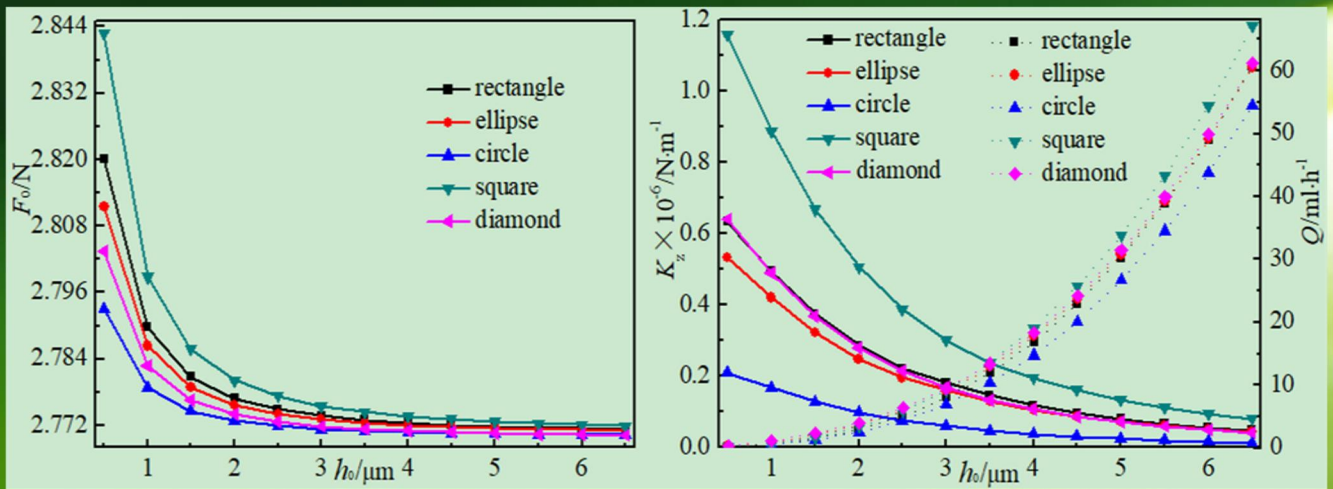
Fig.2 Effect of h_0 on sealing performance parameters
